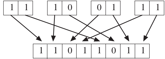
Figure 2: Example of z-order on n-gram vectors.
