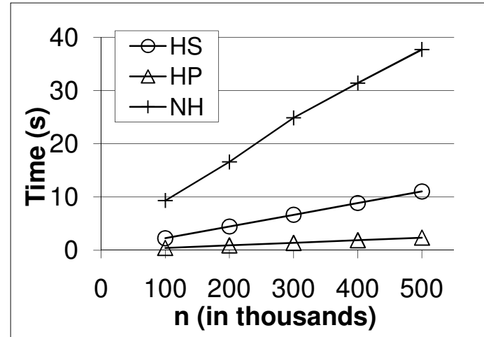
The figure obtained with different parameters ( k=100 , d=7 )
