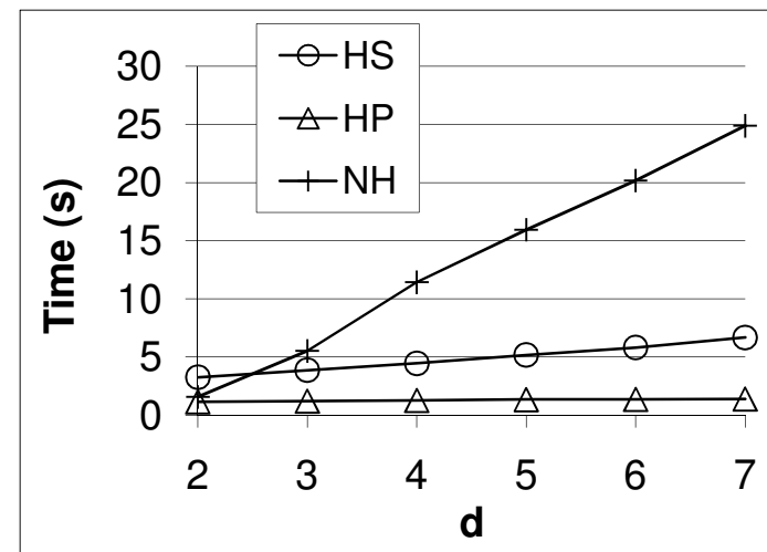
The figure obtained with different parameters ( d= 300K , k=100 )
