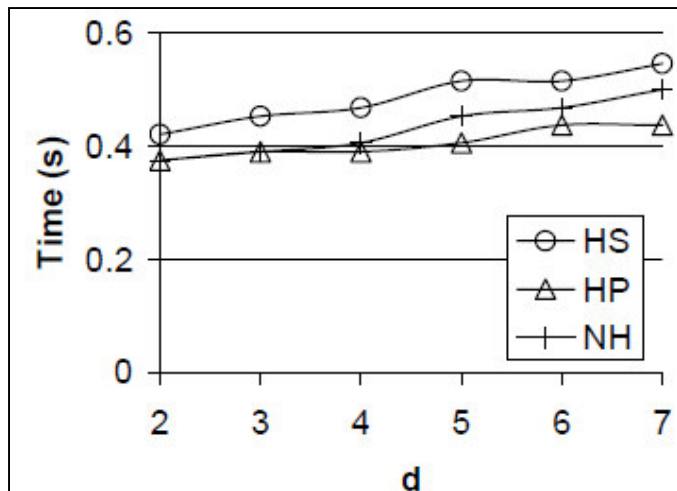
Figure 10 in the paper ( n = 100K , k=10 )
