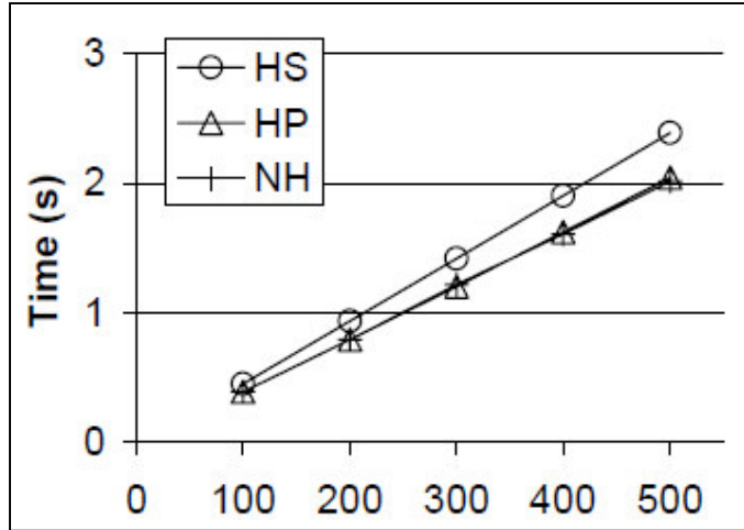
Figure 9 in the paper ( k=10 , d=3 )
