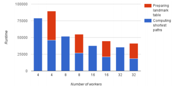
Figure 2: Runtime of shortest-paths computation with and without landmarks computations.
